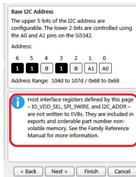
Figure 46. Base I 2 C Address
