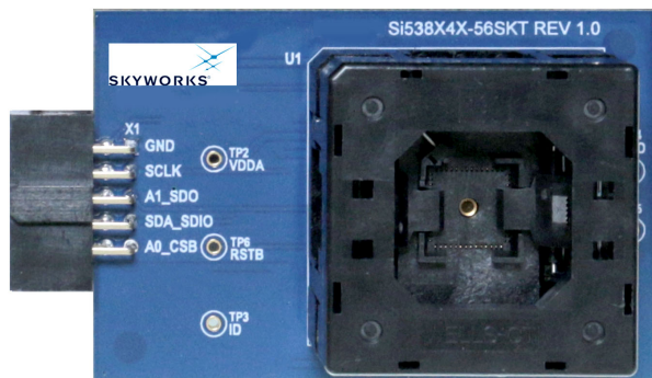
Figure 7. Si538x4x-56SKT-DK
