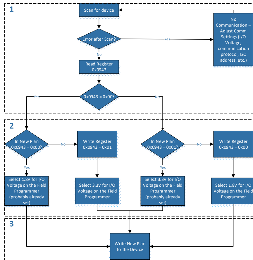
Figure 43. General Steps to Change I/O Power Supply Setting with a Project File
