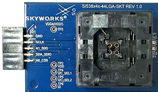
Figure 9. Si538x4x-44LGA-SKT
