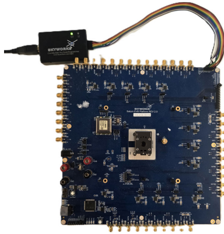
Figure 19. Example I 2 C Connection to External Target Board using Jumper Wires (Si5346-EVB)
