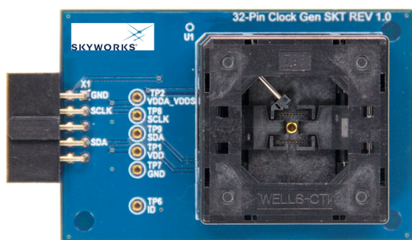
Figure 3. Si533x-32SKT-DK
