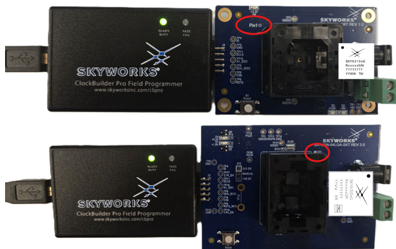
Figure 17. Pin 1 Dot Indicating Device Orientation
