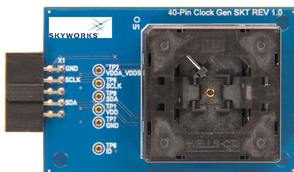
Figure 4. Si5332-40SKT-DK
