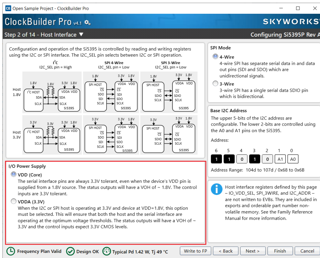
Figure 42. Determine the I/O Power Supply in a CBPro Project
