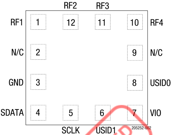
Figure 2. SKY59272-707LF Pinout (Top View)
