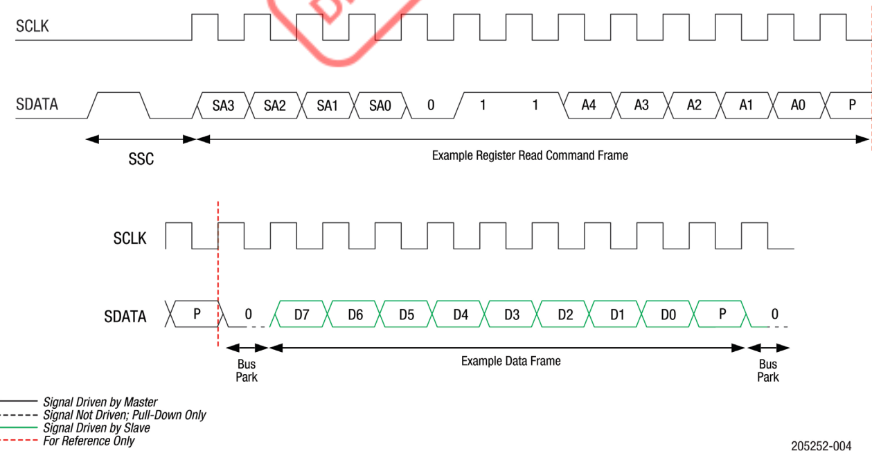
Figure 4. Register Read Command Timing Diagram
