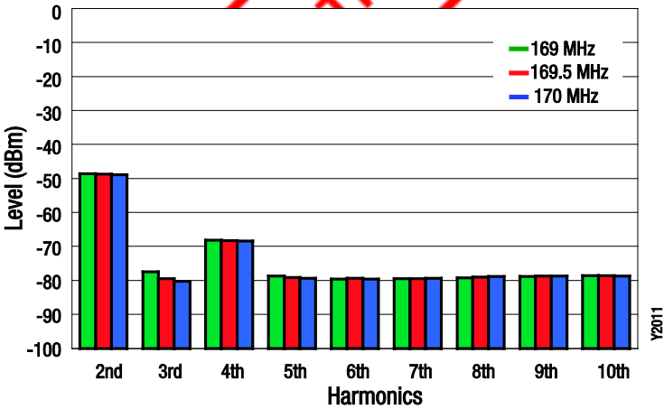
Figure 11. Harmonics at P OUT = +27 dBm
