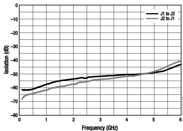
Figure 7. Output to Output Isolation vs Frequency
