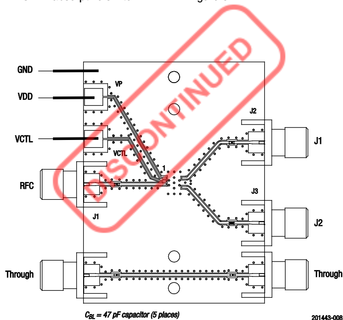
Figure 8. SKY13372-467LF Evaluation Board Assembly Diagram
